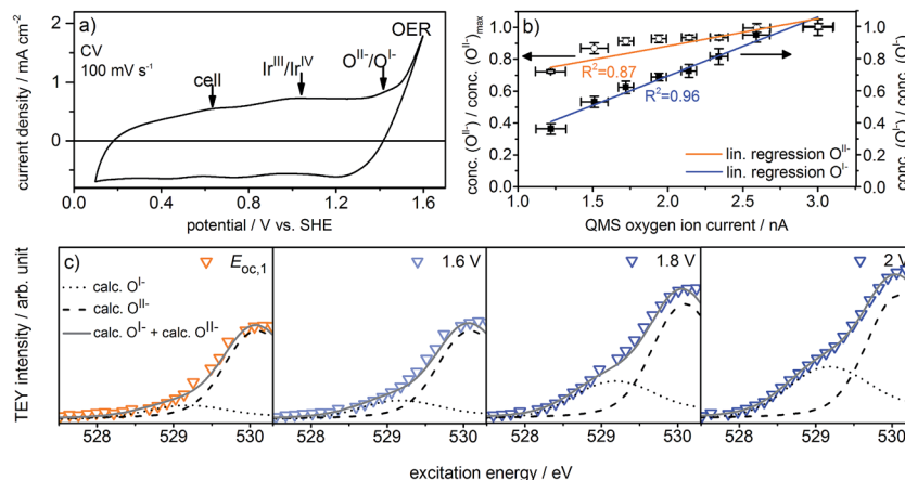
Fig. 2 (a) Cyclic voltammogram, (b) normalized O I and O II concentrations over QMS oxygen ion current, and (c) zoomed and fitted low excitation energy regions of O K-edges recorded in the three-electrode cell (indicated potentials vs. SHE, ring current = 60 mA, p = 0.3 Pa, 0.1 M H 2 SO 4 ).
