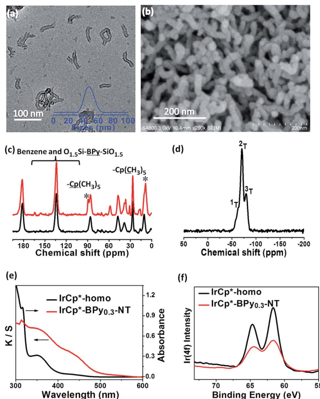
Fig. 2 (a) TEM and (b) SEM images of IrCp*-BP y 0.3 -NT. (c) 13 C CP MAS NMR spectra of BP y 0.3 -NT (black line) and IrCp*-BP y 0.3 -NT (red line). (d) 29 Si MAS NMR spectrum of IrCp*-BP y 0.3 -NT. (e) UV/vis diffuse reflectance spectra and (f) XPS spectra of IrCp*-homo (black line) and IrCp*-BP y 0.3 -NT (red line).
