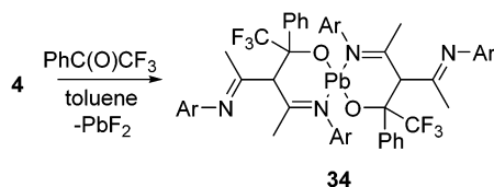
Scheme 12 The reaction of 4 with trifluoroacetophenone (Ar = 2,6- i Pr 2 C 6 H 3 ).
