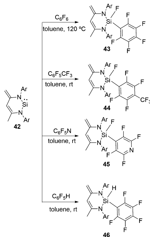
Scheme 15 N-Heterocyclic silylene mediated aromatic C–F bond activation ( \text{Ar} = 2,6\text{-iPr}_2\text{C}_6\text{H}_3 ).
