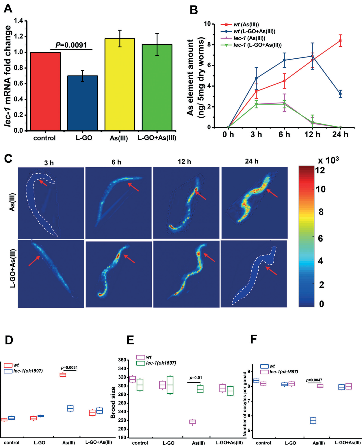
Fig. 8 Effect of LEC-1 in attenuating the toxicity of As(III) by L-GO. (A) Relative levels of lec-1 gene expression to K-medium, L-GO (10 \mu g mL -1 ), and As(III) (10 \mu M) and co-exposure to L-GO and As(III) for 24 h, detected using qRT-PCR analysis ( n = 3 ). (B) As(III) contents in wild type worms and lec-1(ok1597) mutant strain treated with 10 \mu M As(III) and co-exposed for 3, 6, 12, and 24 h, respectively. As(III) contents were determined using ICP-AFS assay ( n = 3 ). (C) As(III) distribution in wild type worms. As(III) (10 \mu M) and L-GO co-exposure for 3, 6, 12, and 24 h. (D) Average apoptotic cells, (E) brood size and (F) number of oocytes per gonad after exposure of wild type worms and mutant lec-1(ok1597) strain to K-medium, L-GO, As(III) and both ( n = 3 ).
