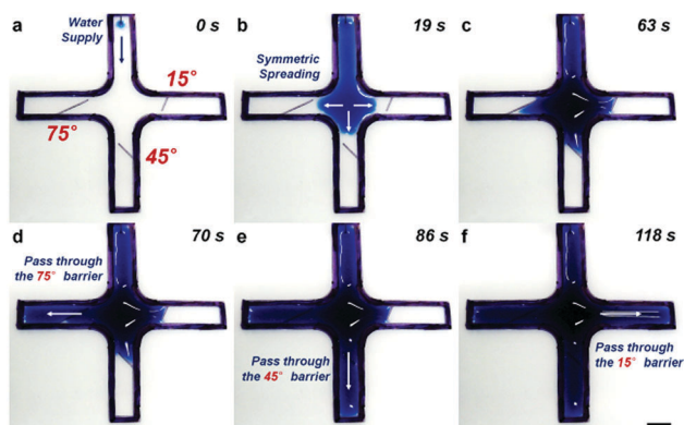
Fig. 4 Ordered liquid delivery on a superhydrophilic surface with branched channels. (a) The spine tilt angles in the various channels. (b) Rapid liquid spreading in the barrier-free channel. (c) Liquid spreading resisted by the barriers. (d–f) Liquid distribution controlled by the tilt angles: liquid firstly passes through (d) the 75^\circ barrier which has the lowest resistance, then (e) the 45^\circ barrier, and finally (f) the 15^\circ barrier. The order of liquid spreading strongly depends on the different motion resistances of the water barriers. Scale bar is 5 mm.
