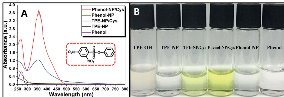
Fig. 5 (A) UV/vis spectra of TPE-NP and phenol-NP solutions (240 \mu\text{M} in PBS/DMSO (v/v = 8/2), pH = 7.4) with and without treatment with Cys and phenol. (B) Photographs of TPE-NP and phenol-NP solutions (240 \mu\text{M} in PBS/DMSO (v/v = 8/2), pH = 7.4) with and without treatment with Cys, TPE-OH and phenol. Inset of part (A) is the structure of phenol-NP.
