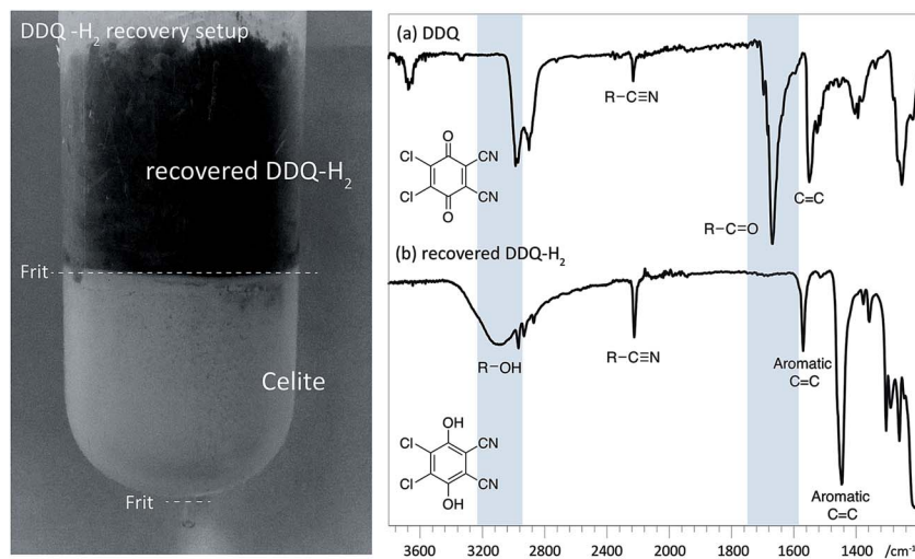
Fig. 8 Left: Recovery of DDQ- \text{H}_2 using celite packed fritted column (See Fig. S24 for colour image†). Right: IR spectra (cropped region) of (a) DDQ and; (b) recovered DDQ- \text{H}_2 . Characteristic differences in the spectra are highlighted with in blue.
