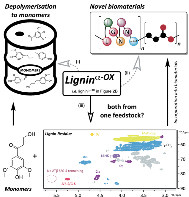
Fig. 9 Applications and approaches to the use of lignin ^{\alpha\text{-OX}} . Route (i) depolymerisation of lignin ^{\alpha\text{-OX}} to monomers (e.g. ref. 6, 8, 32, 50 and 51) and; route (ii) incorporation of lignin ^{\alpha\text{-OX}} into novel biomaterials (e.g. ref. 52 and 53). A different approach (iii) using the same feedstock to produce both monomers and biomaterials has been the key target of this work. Route (iii), using a zinc-mediated depolymerisation approach 8 gives: monomeric keto-alcohol (Fig. S24†) and a soluble lignin residue (inset: 2D HSQC NMR analysis (700 MHz, d_6 -DMSO) of residual beech lignin ^{\alpha\text{-OX}} after zinc reductive cleavage. For coloured contour assignments, see Fig. 2) which through small modifications (e.g. ref. 54) can be used to produce novel biomaterials.
