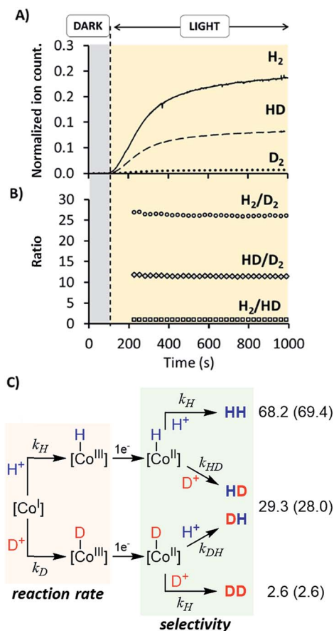
Fig. 10 (A) On-line monitoring of H 2 (solid trace), HD (dashed trace) and D 2 (dotted line) formation vs. time in a MeCN:H 2 O:D 2 O (0.8:0.6:0.6 mL) solvent mixture. (B) Ratios of H 2 /D 2 (dots), HD/D 2 (diamonds) and H 2 /HD (squares) obtained from the ion current data. Conditions: 1 H (50 μM), PS Ir + (150 μM), MeCN:H 2 O:D 2 O (0.8:0.6:0.6 mL), Et 3 N (40 μL), reaction volume = 2 mL, irradiated at λ = 447 nm, under N 2 atmosphere. Ion current response was calibrated with HD and D 2 authentic samples. (C) Heterolytic mechanism for the formation of isotopic distribution of H 2 , DH and D 2 . In parenthesis are the theoretical calculated values.
