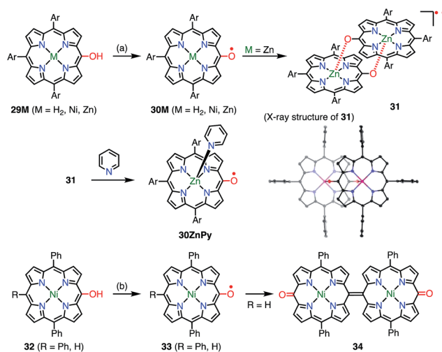
Fig. 11 10,15,20-Triarylporphyrin meso -oxy radicals. (a) 800 equiv. \text{PbO}_2 , \text{CH}_2\text{Cl}_2 , rt, 5 min, 86% for 30H 2 , 91% for 30Ni , 89% for 31 ; (b) aerobic oxidation for 33 , 7 equiv. DDQ, \text{CH}_2\text{Cl}_2 , rt, 30 min, 26% for 34 . Ar = 3,5-di- tert -butylphenyl. Hydrogen atoms and tert -butyl groups in the crystal structure of 31 were omitted for clarity.
