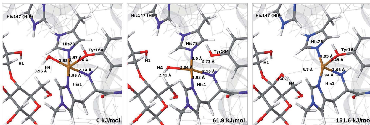
Fig. 13 Reactant 7a (left), transition state (middle) and product 8a (right) for the 7a \rightarrow 8a reaction with His147 is in the HIP state. The structures were optimised with TPSS/def2-SV(P) and energies were obtained with TPSS-D3/def2-TZVPP.
