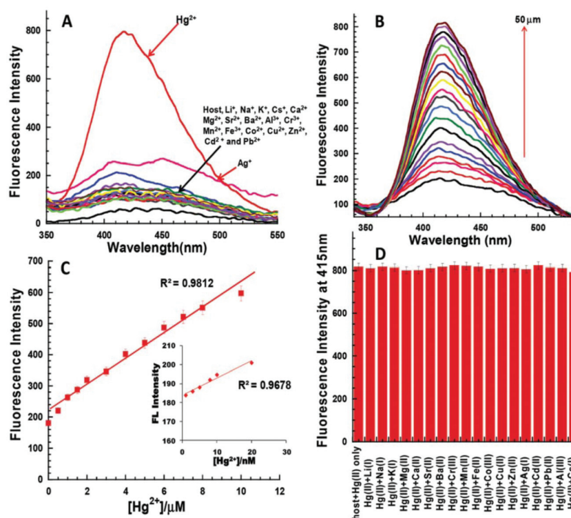
Fig. 15 (A) Changes in the emission profile of nanoaggregates 13 ( 10\ \mu\text{M} ) in water upon the addition of 50\ \mu\text{M} of a particular metal nitrate salt; (B) changes in the emission profile of nanoaggregates 13 ( 10\ \mu\text{M} ) upon the successive addition of \text{Hg}^{2+} ( 0 – 50\ \mu\text{M} ); (C) linear regression graph between the concentration of added mercury ions ( 0 – 10\ \mu\text{M} ) and increase in the fluorescence intensity of nanoaggregates 13 ( 25\ \mu\text{M} ). Inset: Linear regression plot of nanoaggregates 13 ( 10\ \mu\text{M} ) and addition of \text{Hg}^{2+} in the range of 0 – 20\ \text{nM} ; (D) influence of other metal ions on \text{Hg}^{2+} -based changes in the emission profile of nanoaggregates 13 . Adapted with permission from ref. 71. Copyright 2014 the Royal Society of Chemistry.
