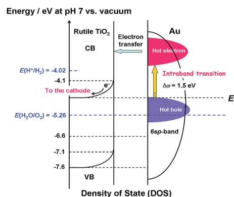
Scheme 2 Energy diagram of the \text{Au}/\text{TiO}_2 plasmonic electrode with the density of states of \text{TiO}_2 and energy distribution of the hot carriers in Au NPs with the intraband transition via the surface plasmon decay.
