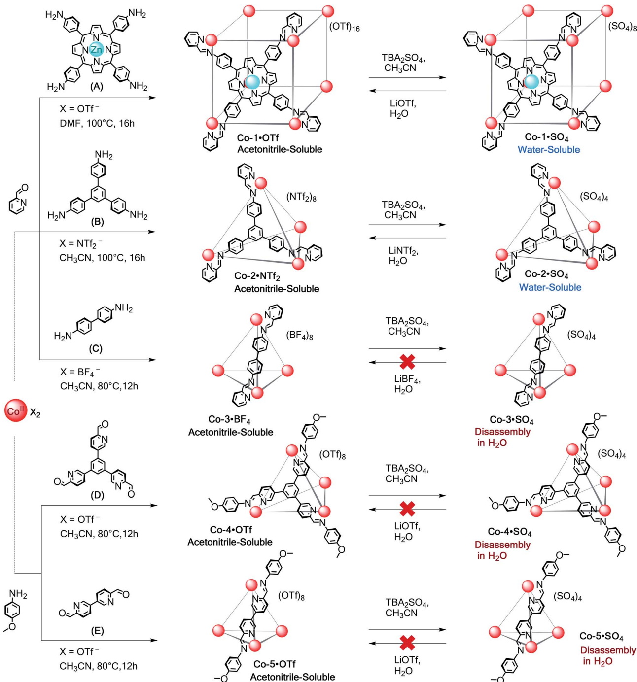
Scheme 1 Subcomponent self-assembly of \text{Co}^{\text{II}} -capsules. Preparation of acetonitrile-soluble Co-1·X to Co-5·X ( \text{X} = \text{OTf}^- , NTf 2 - , or BF 4 - ) from subcomponents A–E and their anion exchange sequences.
