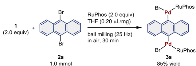
Scheme 3 Gram-scale synthesis of 3s . Conditions: 1 (2.0 mmol), 2s (1.0 mmol), RuPhos (2.0 mmol), and THF (0.20 μL \text{mg}^{-1} ) in a stainless-steel ball-milling jar (25 mL) with two stainless-steel balls (10 mm).
