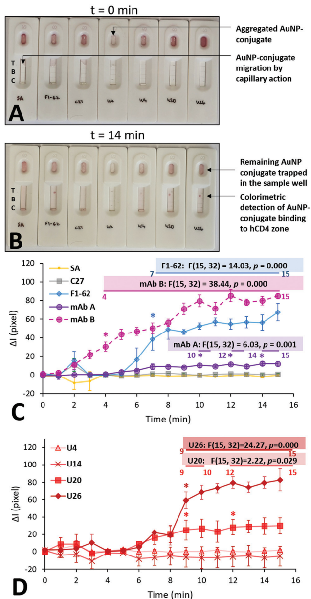
Fig. 6 Multiple time point study evaluating the rate of colorimetric signal generation by the aptamer gold-nanoparticle conjugates on the LFA screening platforms. (A) Initial addition of 50 µL of the various AuNP conjugates; t = 0 min represents the time after the immediate addition of the last U26-AuNP conjugate. (B) Colorimetric detection of hCD4 by the various AuNP conjugates; t = 14 min represents the time after the immediate addition of the last U26-AuNP conjugate. (C) and (D) Comparison of the background-corrected quantified signal intensities at the CD4 zones, caused by the accumulation of the SA-AuNPs functionalized with U4, U14, U20, U26 aptamer and control C27 and F1-62 sequences at a concentration of 0.25 µM. Annotations show the relevant calculated statistics determined using repeated measures ANOVA. The asterisks and the numbered horizontal bars beneath the presented statistics show the times which have been determined to be statistically higher than the baseline ( t = 0 ) responses, as determined using Tukey HSD post hoc tests ( n = 3 separate sensors). Recorded footage of the time point study is shown at 4x speed in Videos S7 and S8.†
