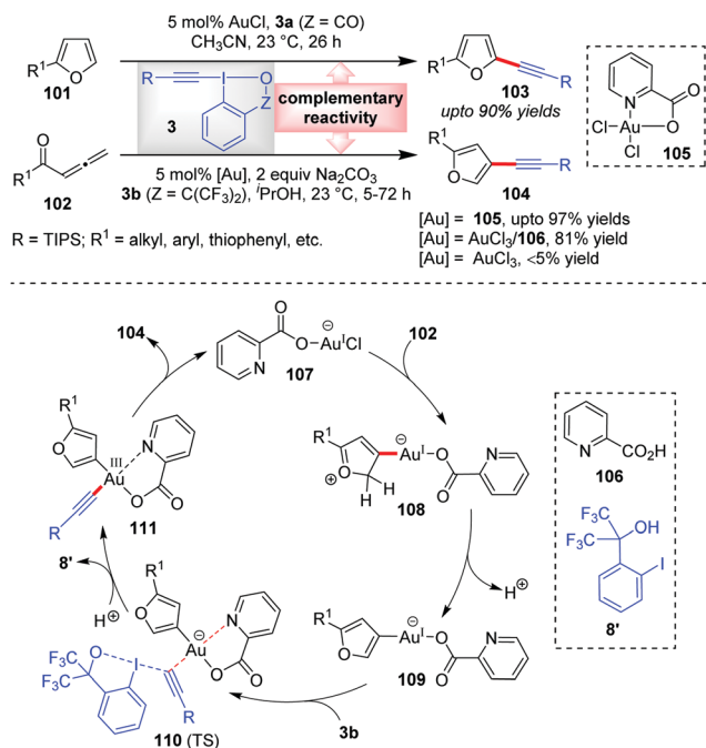
Scheme 17 \pi -Activation mode and interplay mode of Au-catalysis giving rise to regioselective approaches towards C2- and C3-alkynyl furans, respectively.
