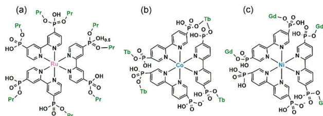
Scheme 9 Coordination modes of metalloligands Ru II (4,4'-dpbpyH 4 ) 3 2+ and [M(5,5'-dpbpyH 4 ) 3 ] n+ .
