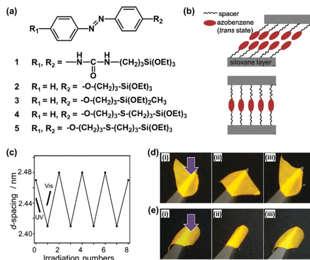
Fig. 4 Soft layered materials based on organopolysiloxane with photomechanical properties. 66–69 (a) Molecular structures of organosiloxanes 1–5 . (b) Schematic illustration of the layered structures derived from the organosiloxanes 4 (upper) and 5 (lower) after hydrolyzation and spin-coating on substrate. (c) Microscopic reversible variation of the interlayer distance, namely d -spacing on the X-ray diffraction pattern, with irradiation of UV and visible lights on the thin-film derived from organosiloxane 4 . (d) and (e) Macroscopic bending and unbending behaviors of a free-standing film derived from the mixture of the organosiloxanes 4 and 5 with UV-vis irradiation from the upper (d) and reverse (e) sides. Reprinted with permission from ref. 66. Copyright 2020 American Chemical Society.
