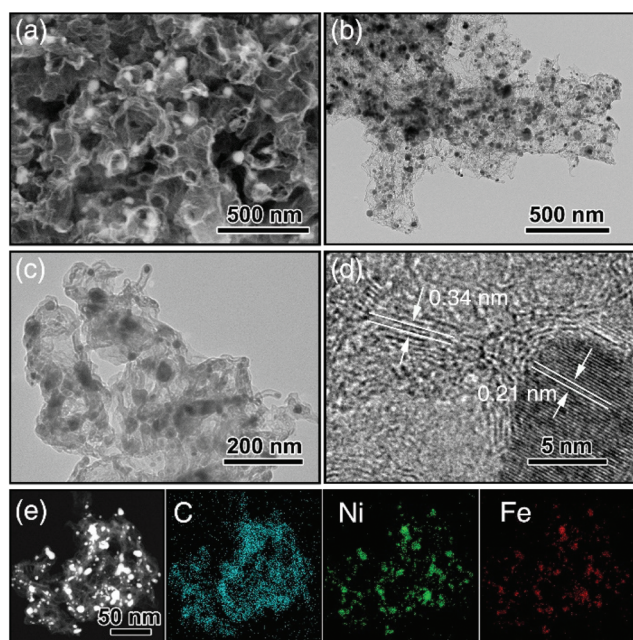
Fig. 1 (a) SEM image, (b and c) TEM images, (d) HRTEM image, and (e) dark-field image of \text{TA-NiFe@NCNT} . Element maps for C, Ni and Fe are also shown in (e).
