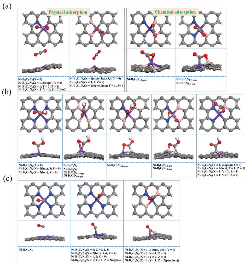
Fig. 3 The different adsorption modes of ^*\text{CO}_2 (a), ^*\text{COOH} (b), and ^*\text{CO} (c) intermediates on Ni-B x C y N z .
