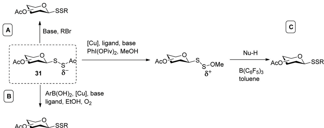
Scheme 11 Different methods to prepare disulfide-linked glycosides from glycosyl dithioperoxyester via: (A) A base-catalysed \text{S}_\text{N}2 process; (B) a copper-catalysed oxidative cross-coupling reaction; (C) an umpolung strategy.
