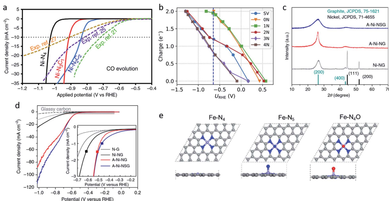
Fig. 3 (a) Calculated j_{\text{CO}} values in the CO 2 RR on Ni-N 2 C 2 , Ni-N 3 C 1 , and Ni-N 4 . Reproduced from ref. 75 with permission from Springer Nature, copyright 2020. (b) Charge capacities of different sites under different potentials for *COOH. Reproduced from ref. 77 with permission from the American Chemical Society, copyright 2020. (c) XRD patterns and (d) LSV curves for A-Ni-NSG, A-Ni-NG, and Ni-NG. Reproduced from ref. 26 with permission from Springer Nature, copyright 2018. (e) Top views and side views of the Fe-N 4 , Fe-N 5 and Fe-N 4 O sites. Reproduced from ref. 78 with permission from Elsevier, copyright 2020.
