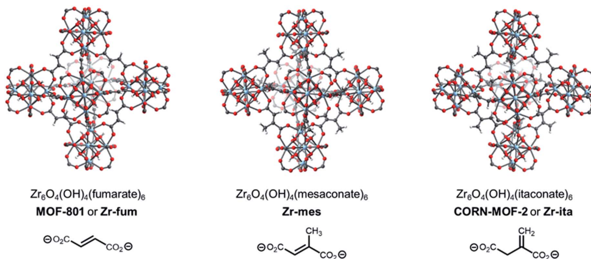
Fig. 1 Density functional theory-calculated ideal structures of known and new sustainably-derived metal–organic frameworks prepared from fumaric, mesaconic, and itaconic acid as part of this work. Gray, white, red, and pale blue spheres correspond to carbon, hydrogen, oxygen, and zirconium, respectively.
