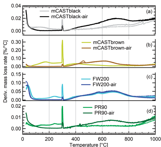
Fig. 17 TGA derivative mass loss rates as a function of temperature ( T ) for fresh and synthetic air ( N_2 + O_2 ) atmosphere oven heated ( 300^\circ C ) bulk soot samples solid and dotted lines indicate two individual TGA runs on the same sample type.
