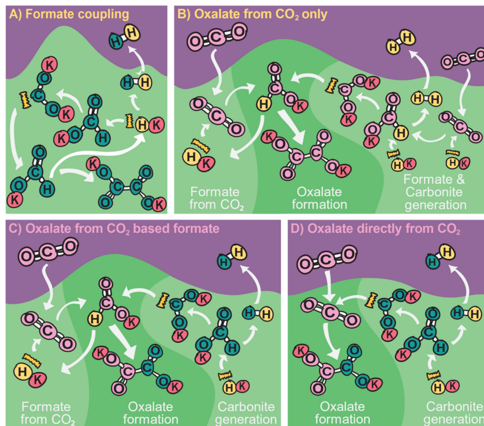
Fig. 16 Three fundamental pathways for oxalate production are consisting of either (A) classic FOCR without the involvement of CO 2 , or (B–D) with the involvement of CO 2 . (A) Oxalate and hydrogen can be formed by traditional formate to oxalate coupling (FOCR) from two formates catalysed by hydride via the carbonite intermediate in the formate melt. CO 2 can dissolve in the formate melt and react towards oxalate in two ways. (B) Two formates can be formed from CO 2 in a reaction between CO 2 and hydride. One of these two formates is activated to carbonite and react with the other formate to oxalate in a FOCR reaction as in (A). (C) It can react with hydride to form formate which can subsequently react towards oxalate in a FOCR reaction. (D) Alternatively, CO 2 can be attacked by the reactive carbonite intermediate formed from the reaction of formate with hydride to form oxalate directly in a stoichiometric reaction.
