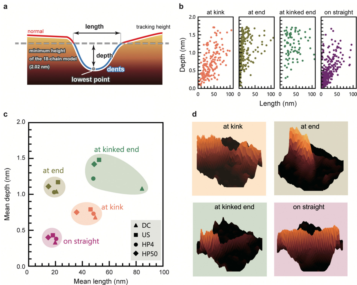
Fig. 4 Morphology of dents. (a) Scheme of length and depth of dents, used as parameters of their morphology, (b) distribution of length and depth of dents at each position. Data corresponding to HP4 is shown here, (c) mean length and depth of defects at each position, plotted for all the samples, (d) 3D views of typical geometry of dents at each position.
