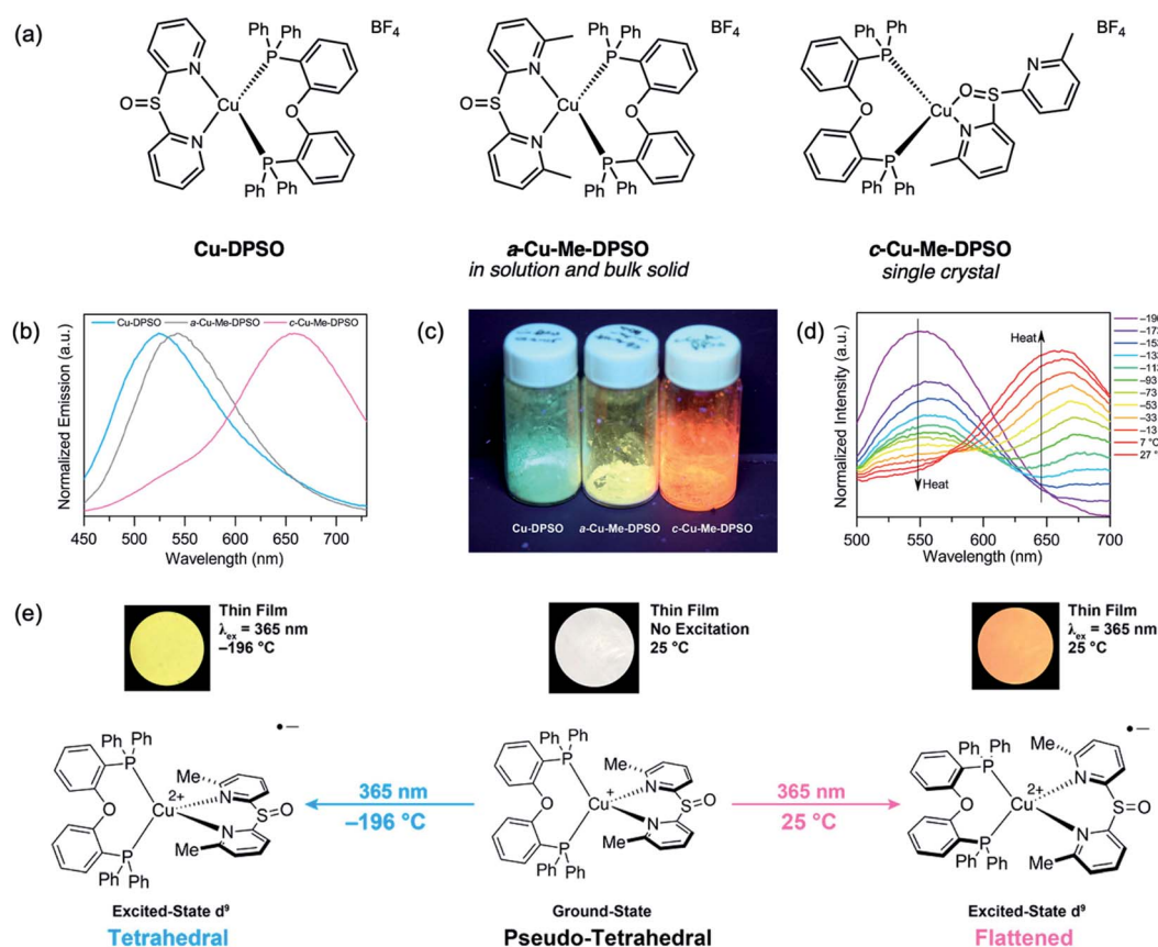
Fig. 18 (a) Structures of Cu(I) complexes \text{Cu-DPSO} and \text{Cu-Me-DPSO} reported by our group. (b) Room-temperature solid-state emission spectra of \text{Cu-DPSO} , a -Cu-Me-DPSO and c -Cu-Me-DPSO (drop-cast from MeOH, \lambda_{\text{ex}} = 390 nm). (c) Photographs of the Cu(I) complexes under UV excitation. (d) Variable-temperature solid-state emission spectra of c -Cu-Me-DPSO from -196 to 27^\circ\text{C} (drop-cast from MeOH, \lambda_{\text{ex}} = 390 nm). (e) Proposed excited-state conformational changes resulting in the thermochromic emission of c -Cu-Me-DPSO. Adapted with permission from ref. 88. Copyright 2018 American Chemical Society.
