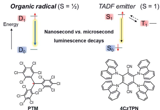
Fig. 2 Comparison of the emission process of the organic radical emitter per -chlorotriphenylmethyl PTM (left) and the TADF emitter 2,3,5,6-tetra(9 H -carbazol-9-yl)terephthalonitrile, 4CzTPN (right). 44
