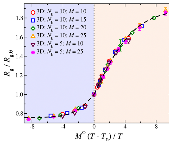
Fig. 4 Average radius of gyration, R_g , of isolated compact nanogel particles normalized by R_{g,\theta} at \theta -point, as a function of the reduced temperature, \tau = (T - T_\theta)/T and chain length, M , scaled with an exponent \varphi . The highlighted regions outline the good solvent conditions for \tau > 0 and poor solvent conditions for \tau < 0 . The uncertainty estimates correspond to two standard deviations. The dashed line is a fit of eqn (4) and the values of the parameters are presented in Table 1.
