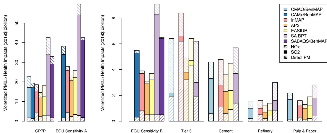
Fig. 6 Monetized \text{PM}_{2.5} health impacts (2019$ billion) for each emissions scenario. Impacts are provided for speciated components of \text{PM}_{2.5} (ammonium nitrate from \text{NO}_x , ammonium sulfate from \text{SO}_2 , and directly emitted \text{PM}_{2.5} ). SA BPT values for the Tier 3 scenario are based on the smallest eastern US BPT value (for Light duty class vehicles) from Table 2 of ref. 39.
