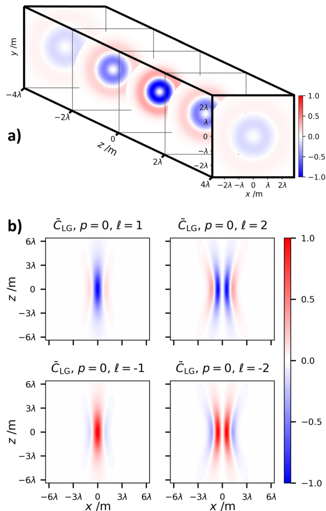
Fig. 9 (a) 3D plot showing the variation of the polarisation independent C_{LG} for a beam with l = 2, p = 0 along the propagation axis. (b) 2D plot showing the diffractive properties of the polarisation independent optical chirality density of LG beams, which stemming purely from longitudinal fields means C_{LG} = \bar{C}_{LG}^{\parallel} . In all plots w_0 = \lambda .
