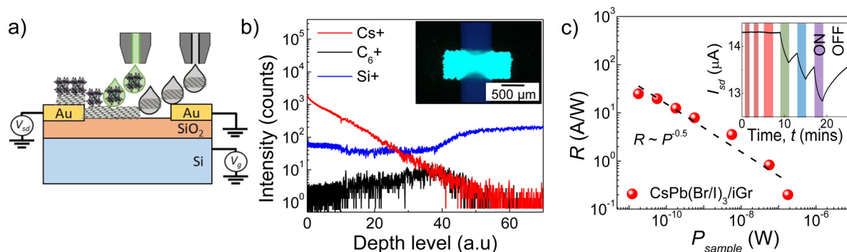
Fig. 4 (a) Schematic of inkjet deposition of perovskite NCs on top of iGr to fabricate fully printed detector. (b) Depth profiling of CsPbBr 3 /iGr heterostructure with 10 printed layers of CsPbBr 3 and 10 printed layers of iGr on Si/SiO 2 substrate via ToF-SIMS. Inset: optical image of CsPbBr 3 /iGr heterostructure on Si/SiO 2 with 10 layers of CsPbBr 3 and 3 layers of iGr under illumination ( \lambda_{\text{ex}} = 365 \text{ nm} ). (c) Photoresponsivity, R , versus power for fully printed CsPb(Br/I) 3 /iGr heterostructure (1 layer CsPb(Br/I) 3 and 1 layer iGr) device with printed AuNP electrodes (1 printed layer) ( \lambda_{\text{ex}} = 520 \text{ nm} illumination, V_{\text{sd}} = 100 \text{ mV} , V_{\text{g}} = 0 \text{ V} ). Inset: temporal response of CsPb(Br/I) 3 /iGr heterostructure device under light illumination ( V_{\text{sd}} = 100 \text{ mV} , V_{\text{g}} = 0 \text{ V} , P = 56.6 \text{ W m}^{-2} ) at different wavelengths: 1060 nm, 808 nm, 635 nm, 520 nm, 450 nm, and 405 nm, respectively.
