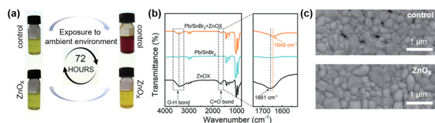
Fig. 5 (a) Photographs confirming oxalate retarding the Sn 2+ oxidation. (b) FTIR spectra and the characteristic regions of pure ZnO x , Pb/SnBr 2 and Pb/SnBr 2 + ZnO x in DMSO. (c) Top-view SEM images of CsPb 0.7 Sn 0.3 IBr 2 thin films with and without ZnO x . Reproduced from ref. 67 with permission from Wiley-VCH, copyright 2022.
