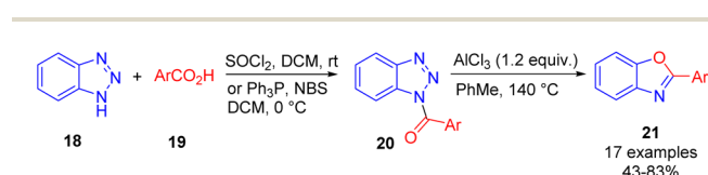
Scheme 14 Synthesis of benzoxazoles from NH-benzotriazoles.
