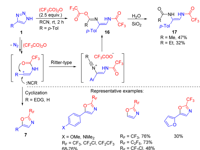
Scheme 13 Formation of bis(enamides) 17 and oxazoles 7 by the cleavage of NH-1,2,3-triazoles with trifluoroacetic anhydride in nitrile solvent.
