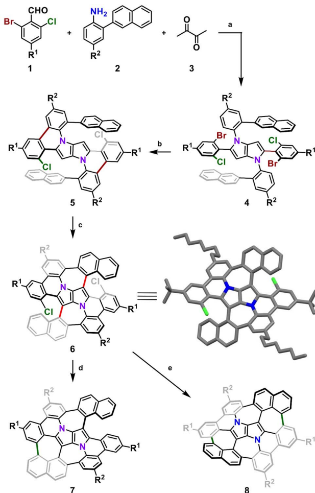
Scheme 1 Synthetic route to molecular saddle 8 . Reagents and conditions: (a) \text{Fe}(\text{ClO}_4)_3 \cdot x\text{H}_2\text{O} (6 mol%), \text{AcOH} /toluene, 50 °C, 16 h, 49%; (b) \text{Pd}(\text{OAc})_2 (20 mol%), \text{Cs}_2\text{CO}_3 (2.4 equiv.), \text{PPh}_3 (48 mol%), toluene, 120 °C, 4 h, 91%; (c) \text{Fe}(\text{OTf})_3 (6.0 equiv.), \text{DCE}/\text{MeNO}_2 , 80 °C, 6 h, 24%; (d) \text{Pd}(\text{OAc})_2 (2.0 equiv.), \text{HPt-Bu}_2\text{MeBF}_4 (6.0 equiv.), \text{DBU}/\text{DMA} , 180 °C, 24 h, 52%; (e) t\text{-BuOK} (10.0 equiv.), \text{DMSO} , blue LEDs, rt, 20 h, 75%. \text{DMA} – dimethylacetamide, \text{DCE} – 1,2-dichloroethane; inset: X-ray crystal structure of 6 . \text{R}^1 = t\text{-Bu} , \text{R}^2 = n\text{-C}_8\text{H}_{17} .
