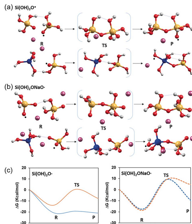
Fig. 3 Optimized geometries of the structures involved in the condensation of (a) \text{Si}(\text{OH})_3\text{O}^\bullet and (b) \text{Si}(\text{OH})_2\text{ONaO}^\bullet radical species with \text{Si}(\text{OH})_3\text{ONa} and \text{Al}(\text{OH})_4\text{Na} . Si, Al, O, H, and Na atoms are depicted as yellow, blue, red, white and purple spheres, respectively. (c) Corresponding Gibbs free energy profiles for condensation of radicals with \text{Si}(\text{OH})_3\text{ONa} (blue) and \text{Al}(\text{OH})_4\text{Na} (orange). Reproduced from ref. 50 with permission from Wiley, Copyright 2020.
