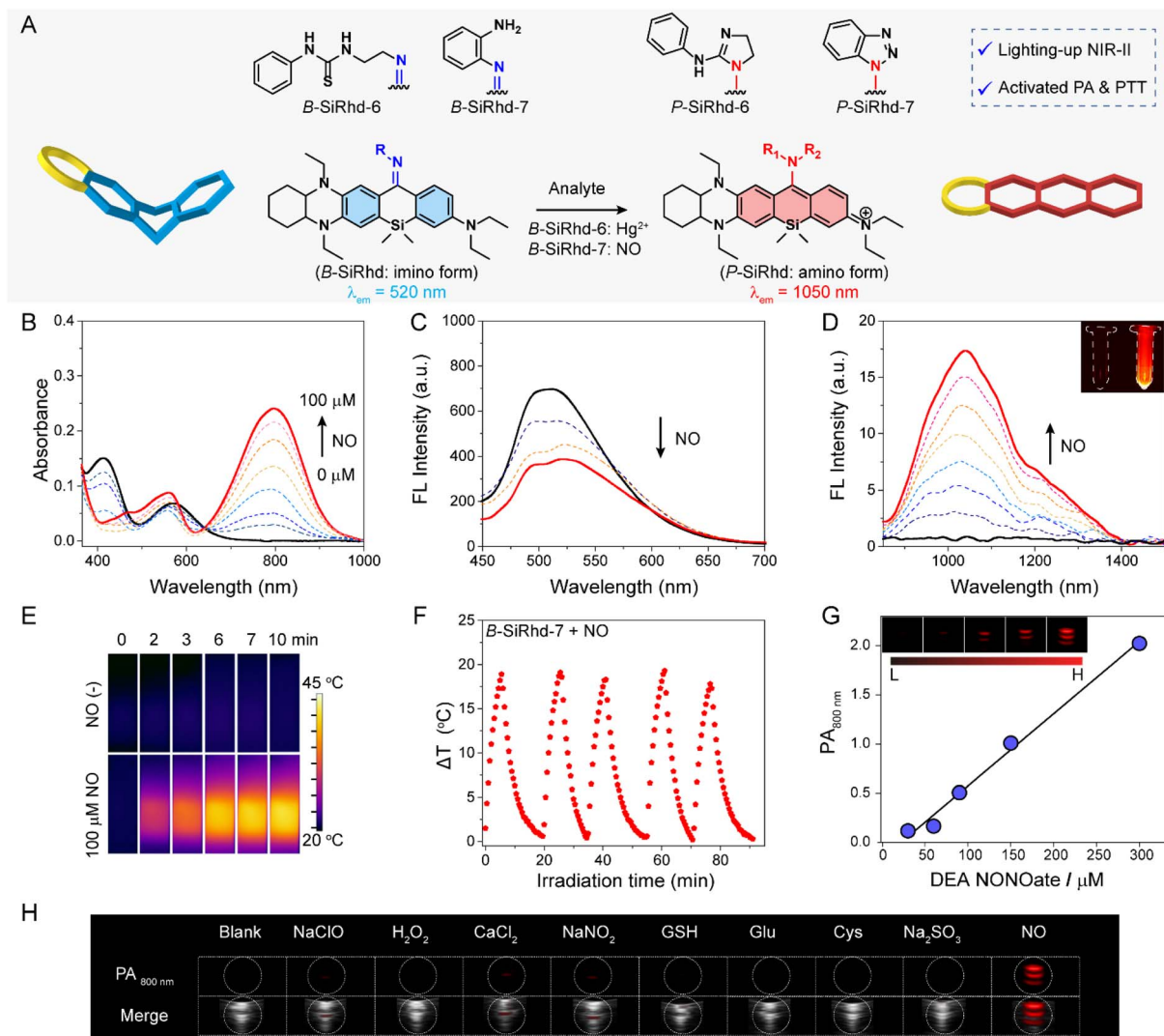
Fig. 5 The molecular bent-to-planar strategy for lighting-up NIR-II sensing. (A) Schematic illustration of the sensing mechanism for B-SiRhd-6 and B-SiRhd-7 towards Hg 2+ and NO, respectively. Activatable NIR-II response: absorption (B) and fluorescence emission (C and D) spectra of B-SiRhd-7 (10 μM) in the presence of NO in a mixed solution. (E) Photothermal activation: thermal infrared image of B-SiRhd-7 (20 μM) in the presence of NO under 808 nm laser irradiation (2 W cm -2 ). (F) Excellent photothermal stability: the variation of temperatures during five cycles of heating-cooling processes under 808 nm laser irradiation of B-SiRhd-7 (20 μM) with 100 μM NO. (G) Photoacoustic (PA) activation: plot of PA 800 nm of B-SiRhd-7 against the concentration of NO. (H) In vitro PA images of the solution of B-SiRhd-7 in the presence of various biologically relevant species at 800 nm.
