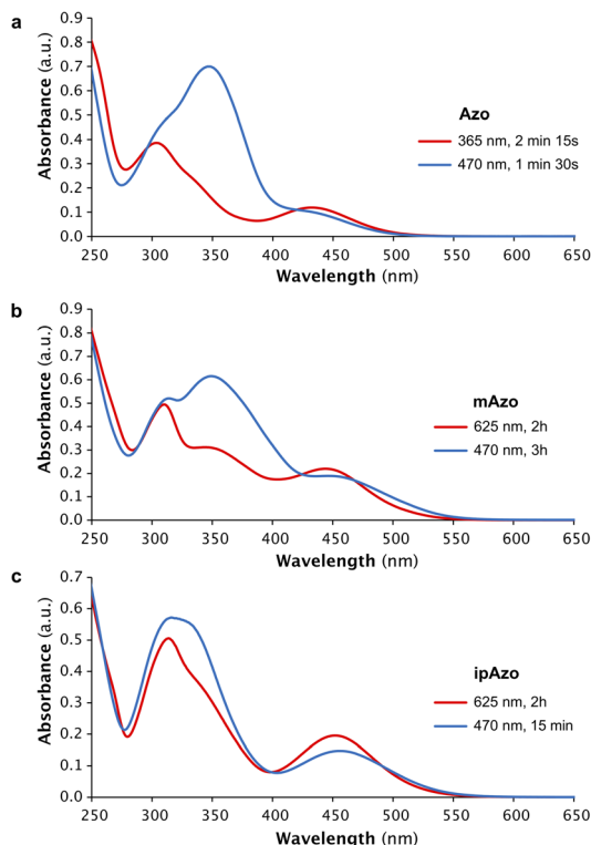
Fig. 2 UV-vis absorption spectra of templates (a) Azo , (b) mAzo , and (c) ipAzo ( 50\text{ }\mu\text{M} in 100\text{ mM} sodium phosphate buffer at \text{pH } 7.5 ) showing the photostationary states at the specified wavelengths. The irradiation times required to obtain the different photostationary states are indicated. The spectra showing primarily the cis and trans isomers are depicted in red and blue, respectively.
