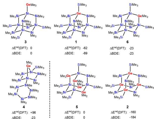
Fig. 3 Relative energies \Delta E^{\text{rel}}(\text{DFT}) , in kJ mol ^{-1} , of selected \text{Si}_{13}\text{Ge}_1\text{-Me}_{24} and \text{Si}_{10}\text{Ge}_4\text{Me}_{24} isomers. Both calculated at M06-2X/6-311+G(d,p) and estimated on the basis of bond dissociation energies \Delta \text{BDE} .
