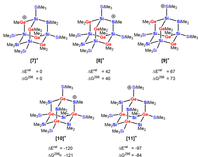
Fig. 4 Relative energies \Delta E^{\text{rel}} and free enthalpies \Delta G^{298} of \text{Si}_{10}\text{Ge}_4\text{-Me}_{23} cations derived from heteroadamantanes 3 ([7] ^{+} –[9] ^{+} ) and 4 from ([10] ^{+} , [11] ^{+} ), in kJ mol ^{-1} , at M06-2X/6-311+G(d,p).
