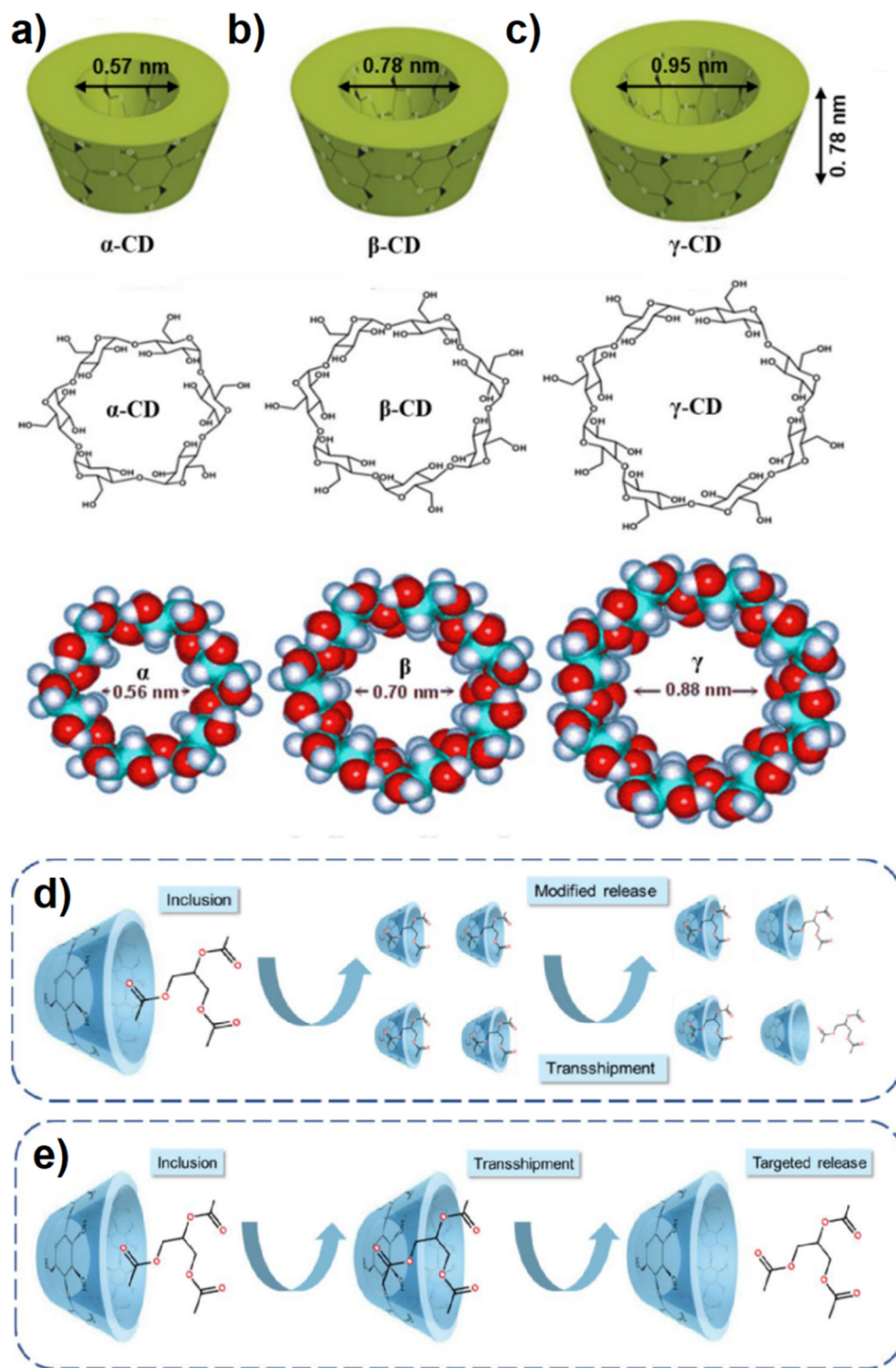
Fig. 11 The structures of α- (a), β- (b) and γ-CD (c), schematic diagram of CD-based sustained release. In the first step, a mixture of CD and core material leads to the inclusion complex formation. In the second step, movement of the inclusion complex to an area of low core material concentration leads to a relatively slow release of the core material (d), schematic diagram of CD-based targeted release. In the first step, a mixture of CD and core material leads to the inclusion complex formation. In the second step, movement of the inclusion complex to a specific area that differs in pH or reducing potential or other triggering phenomenon causes release of the core material (e). Reproduced from ref. 117 with permission from Taylor & Francis.
