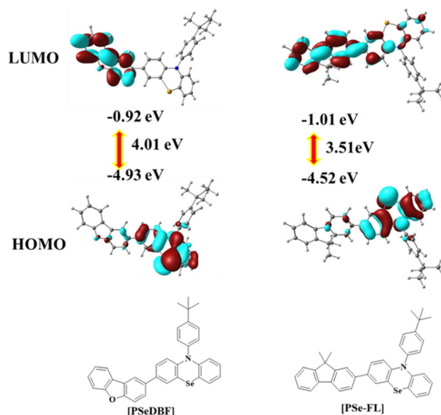
Fig. 1 Frontier orbitals distributions of PSeDBF and PSeFL.
