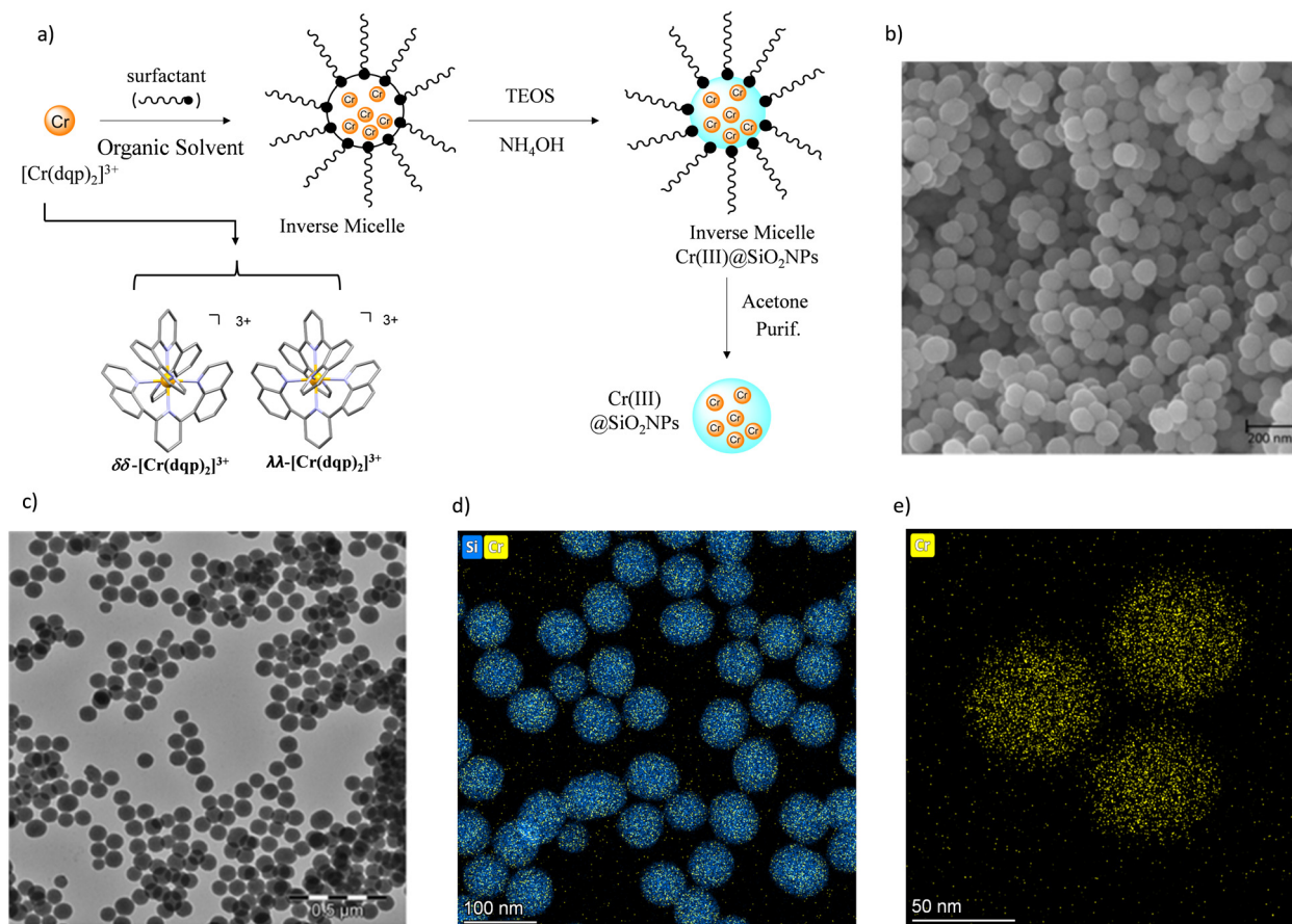
Fig. 3 (a) Schematic synthetic approach for preparing the silica nanoparticles (b) SEM image of the prepared \text{rac-Cr}@\text{SiO}_2\text{NPs} (c) TEM image of the prepared \lambda\lambda\text{-Cr}@\text{SiO}_2\text{NPs} ; (d) and (e) HAADF-STEM compositional mapping image of \lambda\lambda\text{-Cr}@\text{SiO}_2\text{NPs} .
