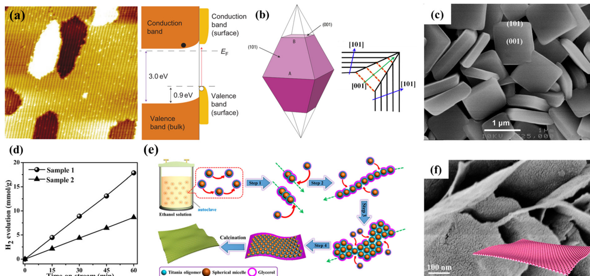
Fig. 7 (a) Atomic-resolution scanning tunnel microscopy images of the (011) surface of \text{TiO}_2 rutile and its band diagram. Reprinted with permission from ref. 49. Copyright © 2011, The Nature Publishing Group. (b) Scheme of the growth of (001) and (101) facets of \text{TiO}_2 anatase. Red line: rapid growth; black line: slow growth. Reprinted with permission from ref. 51, Copyright © 1969, The Nature Publishing Group, and 54, Copyright © 2015, Springer Nature. (c) SEM image of \text{TiO}_2 nanosheets. Reprinted with permission from ref. 56. Copyright © 2009, American Chemical Society. (d) \text{H}_2 production of \text{TiO}_2 nanosheets under UV light with different percentages of reactive (001) facets (Sample 1–97%, Sample 2–68%). Reprinted with permission from ref. 58. Copyright © 2017, Wiley-VCH. (e) Schematic illustration of the formation process and (f) SEM image of the single-layered 2D ordered mesoporous \text{TiO}_2 nanosheets using a hydrothermal-induced solvent-confined monomicelle assembly. Reprinted with permission from ref. 61. Copyright © 2018, American Chemical Society.
