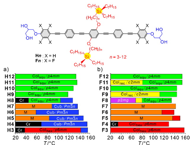
Fig. 2 Molecular structure and LC phases of (a) H n and (b) F n as observed on cooling with 10 K min −1 ; abbreviations: Cr = crystalline solid; Col hex /p6mm and Col squ /p4mm = triangular and square LC honeycombs, respectively; Col rec /c2mm and p2mg = tilings by rhombic and non-regular triangular honeycombs, respectively; Cub/Pm3n = cubic network phase with Pm3n space group; M = unknown LC phases; isotropic liquid is at the right side of the columns; for numerical data, transitions on heating and enthalpies, see Table S1a, b, for DSCs Fig. S1 and S2, for textures Fig. S3–S6, for SAXS/WAXS data Fig. S7–S10, Tables S2–S29 (ESI†).
