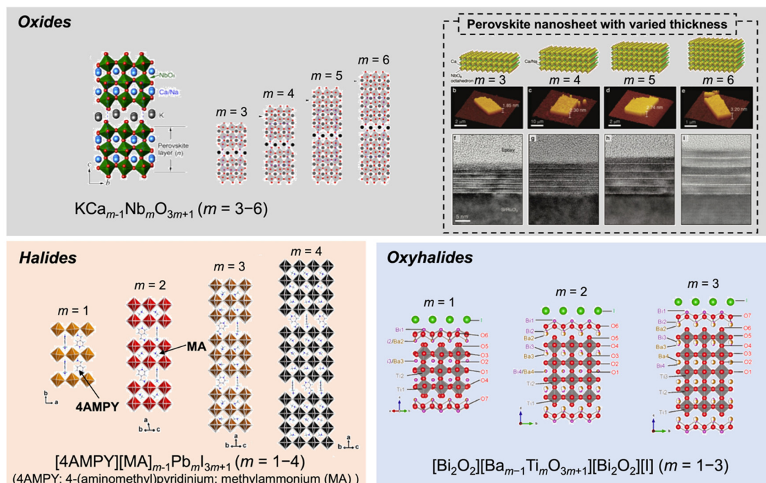
Fig. 34 Structural and compositional variation in perovskite-type layered compounds; oxides, 547,551 hallides 593 and oxyhalides. 594
