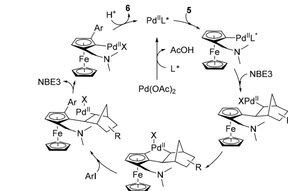
Scheme 8 Proposed reaction mechanism for the remote asymmetric functionalisation of ferrocene using a transient mediator.
