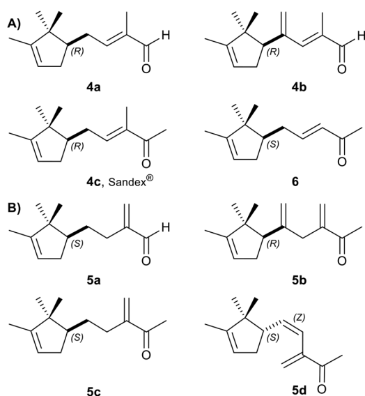
Fig. 1 Substrates submitted to bioreduction: (A) α,β-unsaturated carbonyl compounds; (B) α-methylene isomers.
