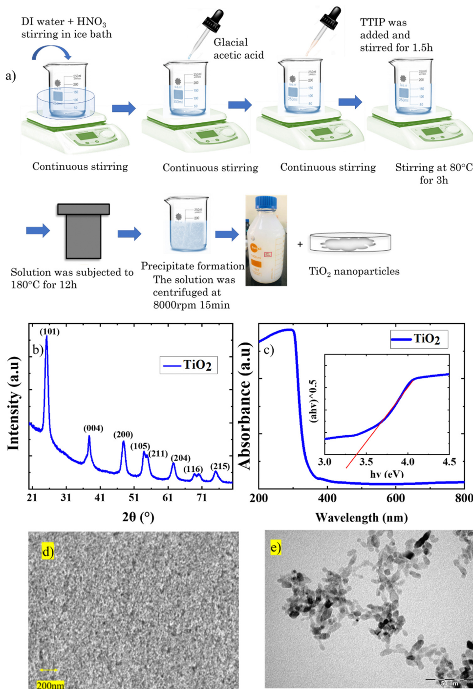
Fig. 1 (a) Schematic representation of uniformly dispersed anatase TiO 2 sol and nanoparticle synthesis, (b) XRD spectra, (c) absorbance spectra (d) FE-SEM images and (e) TEM of TiO 2 films fabricated from TiO 2 sol.
