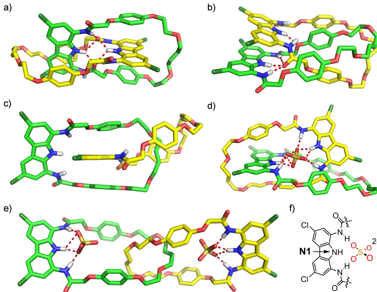
Fig. 11 Low-energy conformations (a–c) of free catenane A obtained from conformational search. Snapshots from MD simulations showing stable conformations of (d) \text{A} \times \text{SO}_4^{2-} and (e) \text{SO}_4^{2-} \times \text{A} \times \text{SO}_4^{2-} . (f) Atom labels used in the discussion of MD simulations.
