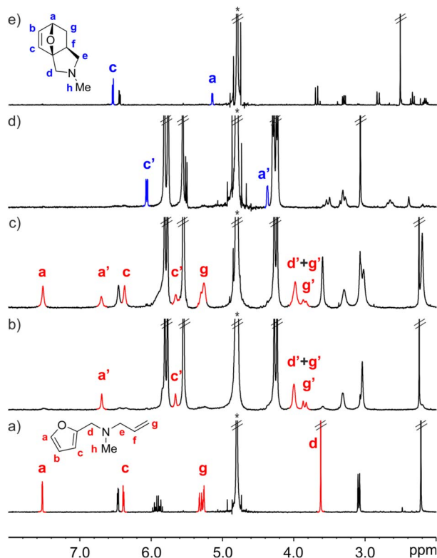
Fig. 2 Selected region of the 1 H NMR spectra (400 MHz, D 2 O, 298 K) of: (a) FA-1 (0.005 M); (b) FA-1 ⊂ CB[7] (1.05 : 1, 0.005 M); (c) FA-1 ⊂ CB[7] (2 : 1, 0.005 M); (d) P-1 ⊂ CB[7] (1 : 1, 0.005 M), acquired after 16 h of evolution of spectrum b; and (e) P-1 (0.005 M). FA-1 in red and P-1 in blue. Primed labels correspond to proton signals of bound species. *Residual solvent peak.
